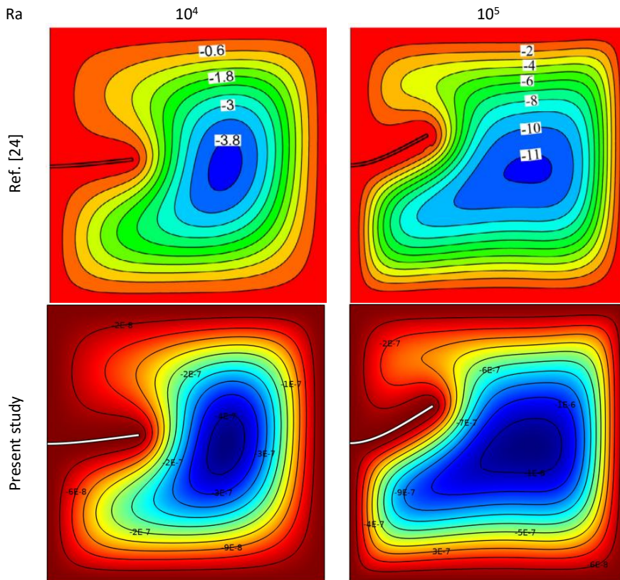
Figure 4. Comparison of the results obtained in the present study and the streamlines reported in literature [24] when Pr = 10 and Et = 10^{10}
