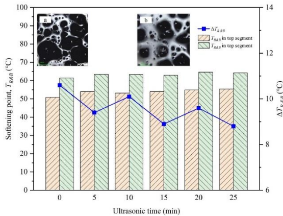
Figure 8. Segregation experimental results and OSM morphology of crumb rubber modified asphalt under different ultrasonic cooperative mixing process.
