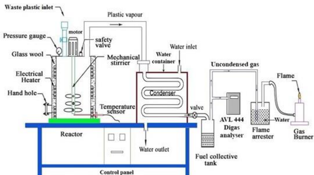
Figure S1. The pyrolysis plant's schematic design.
